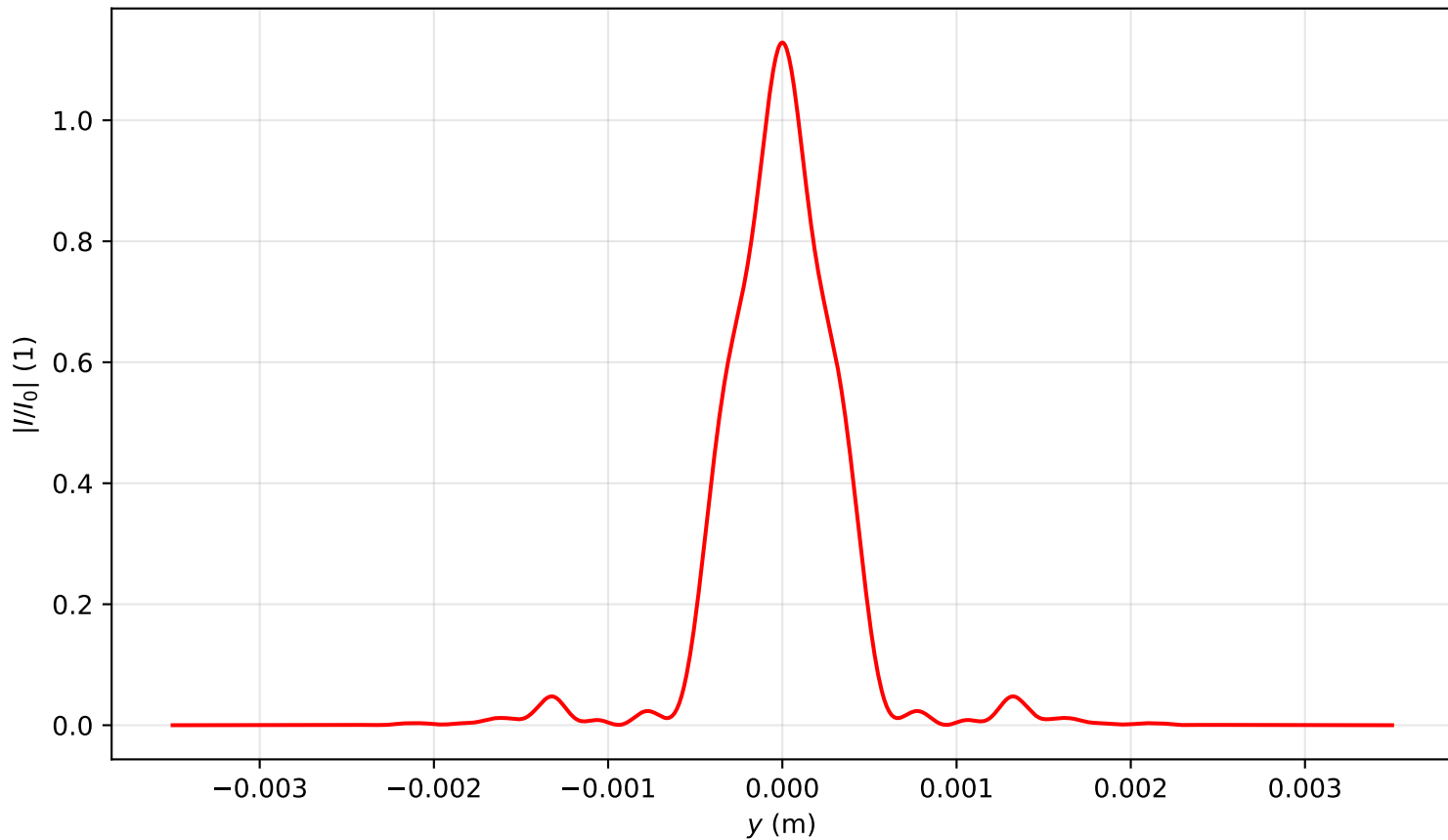
Intensity profile I(x=0, y, z=1.911)/I_0 , P_{in}=3.5P_{cr} , artificial time
